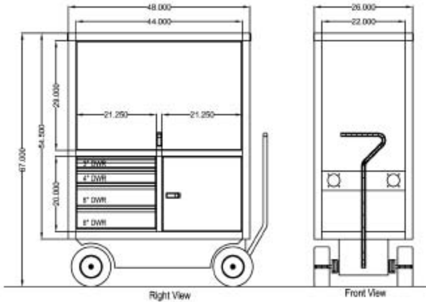
Right View
